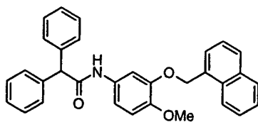
Compound # 49
